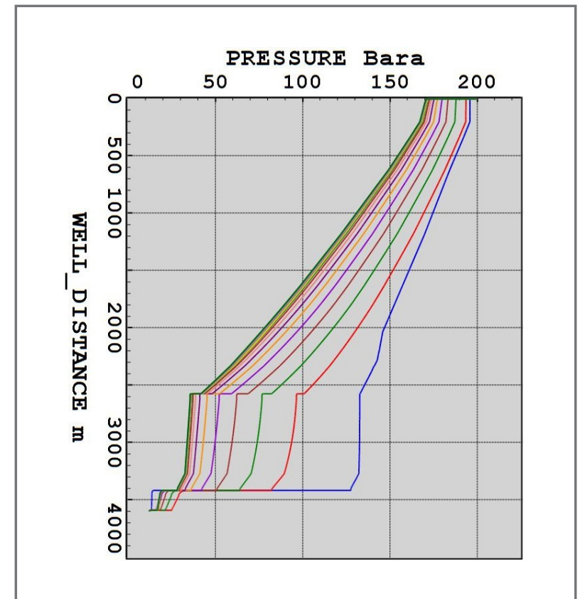
A transient well start-up simulation from cold conditions showing pressure profiles along the well.
