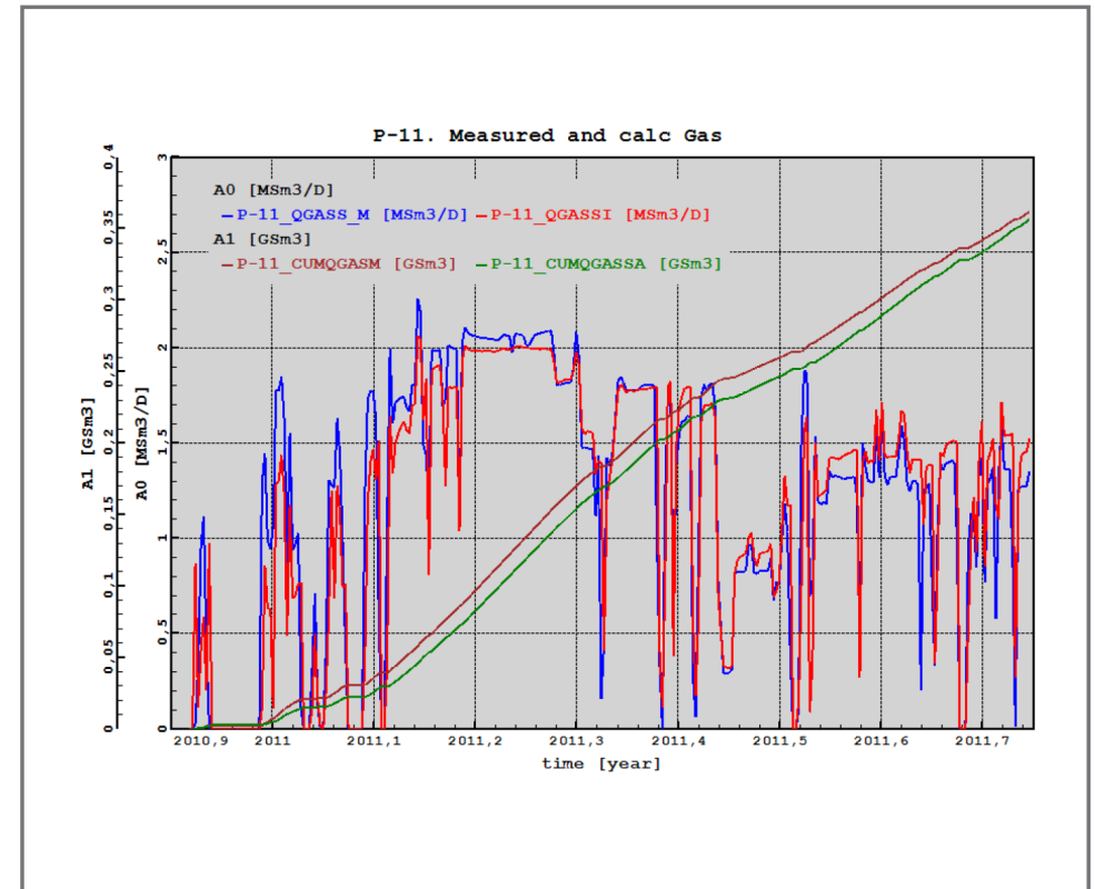
Virtual flow metering is applied to a gas producing well (P-11) comparing reference gas rate in blue with estimated gas rate from Aspen METTE in red.
